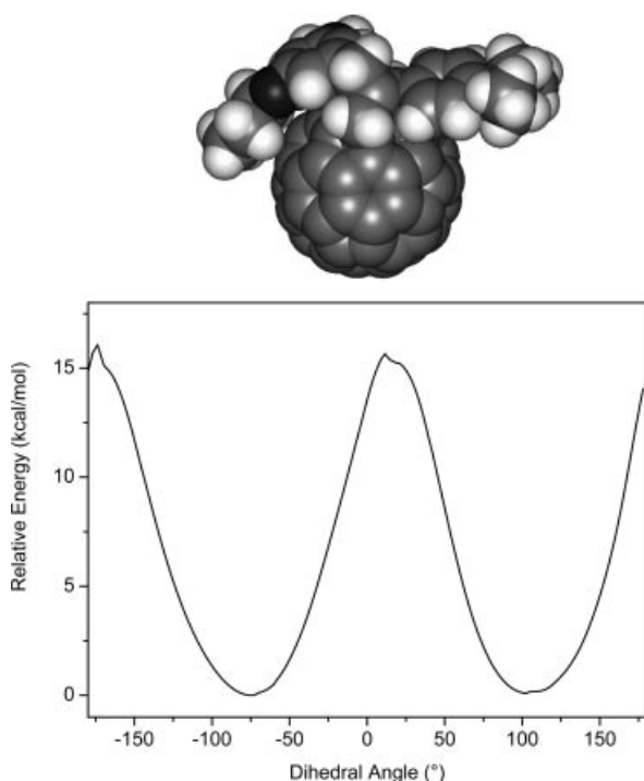
Figure 2. Bottom: calculated potential energy diagram of compound 5b for rotation about the bond between the pyrrolidine ring and the phenyl group attached to it (the dodecyl chains have been replaced by propyl chains in the calculations). Top: theoretical structure of the most stable conformer.
