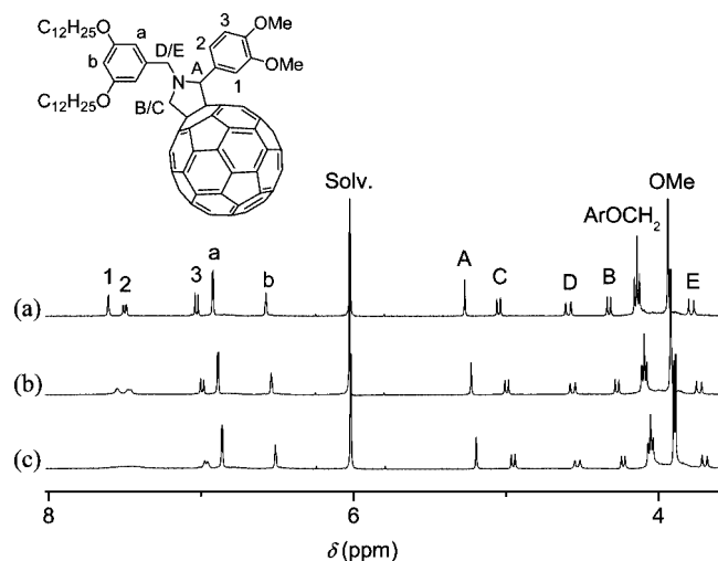
Figure 6. 1 H NMR spectra (400 MHz, CDCl 2 CDCl 2 ) of 5d recorded at 100 °C (a), 50 °C (b) and 30 °C (c).
