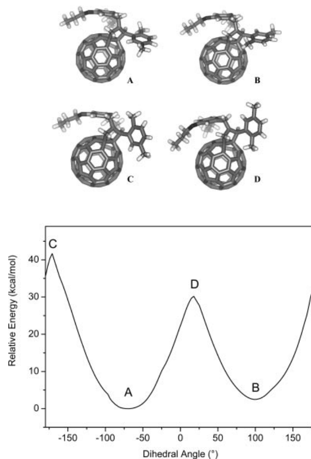
Figure 5. Bottom: calculated potential energy diagram of compound 5g for rotation about the bond between the pyrrolidine ring and the phenyl group attached to it (the dodecyl chains have been replaced by propyl chains in the calculations). Top: theoretical structures of the four conformers corresponding to the two minima ( A and B ) and the two maxima ( C and D ).
