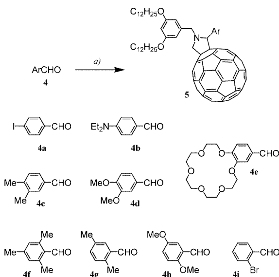
Scheme 2. Reagents and conditions: (a) \text{C}_{60} , 3 , ODCB, 180 °C (34–54%).
