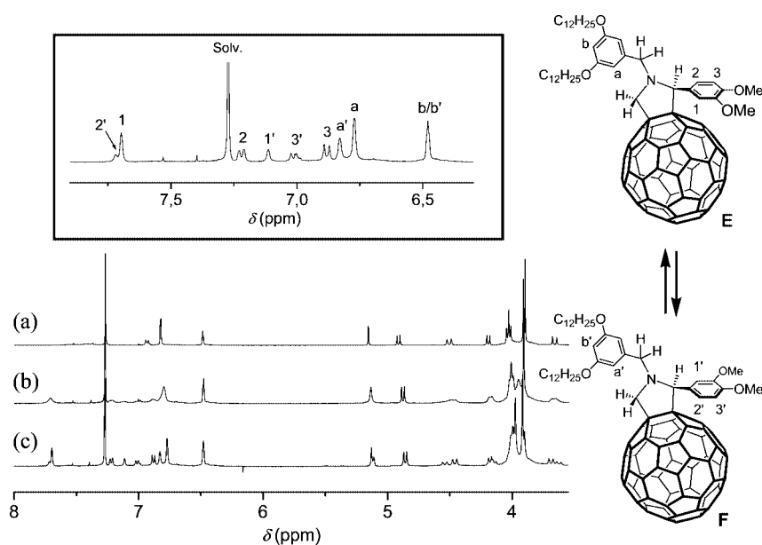
Figure 7. 1 H NMR spectra (400 MHz, CDCl 3 ) of 5d recorded at 20 °C (a), -10 °C (b) and -40 °C (c). Inset: aromatic region of the spectrum recorded at -40 °C.
