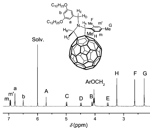
Figure 3. ^1\text{H} NMR spectrum (400 MHz, \text{CDCl}_2\text{CDCl}_2 ) of 5f recorded at room temperature.
