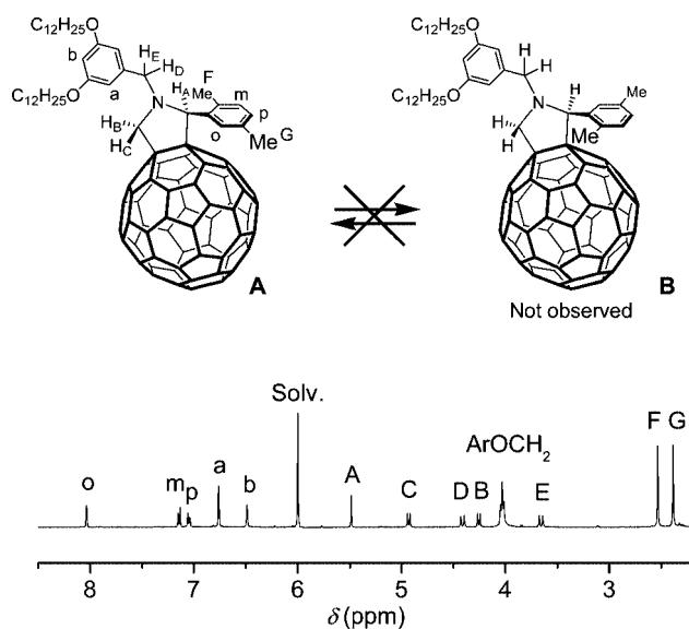
Figure 4. ^1\text{H} NMR spectrum (400 MHz, \text{CDCl}_2\text{CDCl}_2 ) of 5g recorded at room temperature.
