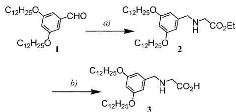
Scheme 1. Reagents and conditions: (a) glycine ethyl ester hydrochloride, \text{Et}_3\text{N} , EtOH, THF, molecular sieves (3 Å), room temp., then \text{NaBH}_4 , 0 °C to room temp. (79%); (b) KOH, \text{H}_2\text{O} , EtOH, THF, room temp., then HCl (99%).
