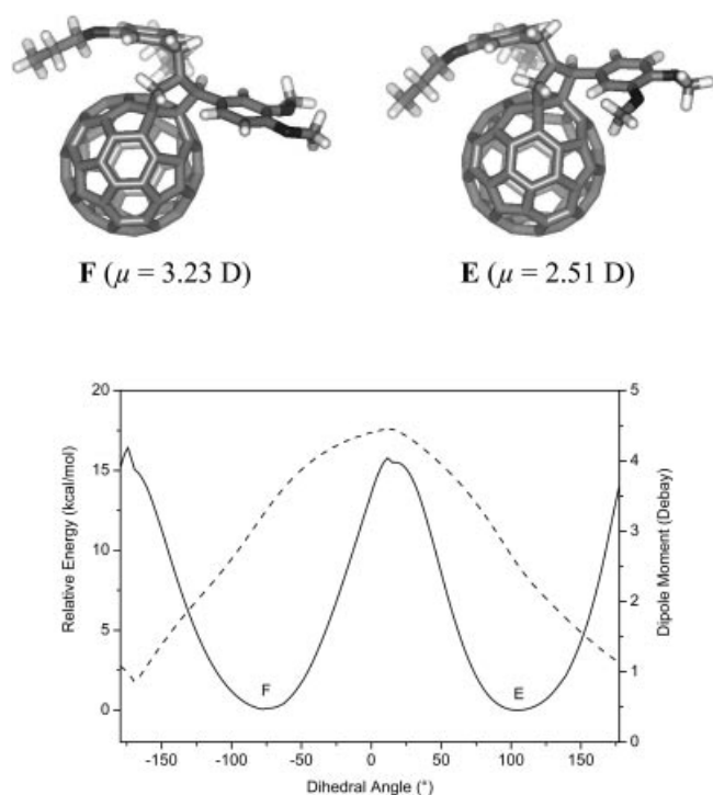
Figure 8. Bottom: calculated potential energy diagram (full line) of compound 5d for rotation about the bond between the pyrrolidine ring and the phenyl group attached to it and calculated dipole moment (dotted line) as a function of the dihedral angle (the dodecyl chains have been replaced by propyl chains in the calculations). Top: theoretical structures of the two conformers corresponding to the two minima ( E and F ).
