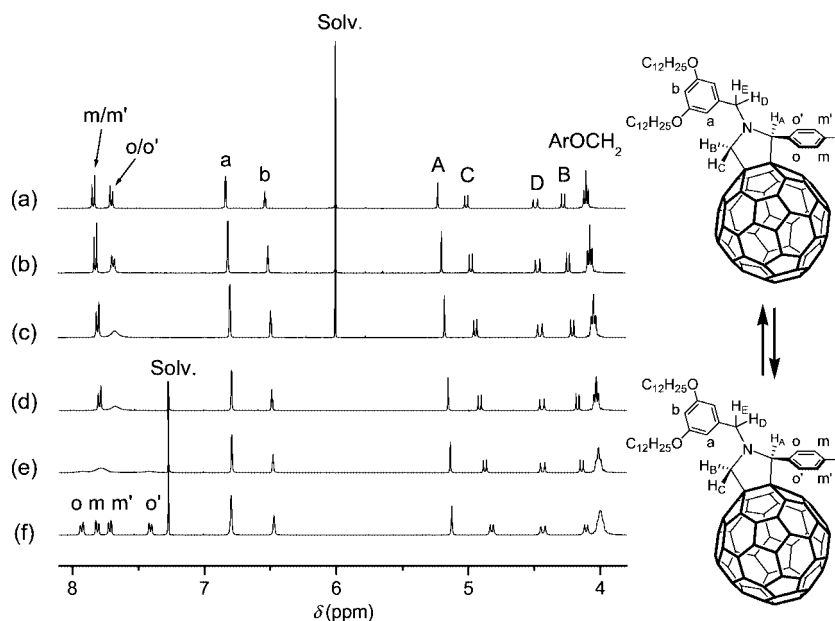
Figure 1. ^1\text{H} NMR spectra (400 MHz) of 5a recorded in \text{CDCl}_2\text{CDCl}_2 at 100 °C (a), 50 °C (b) and 30 °C (c) and in \text{CDCl}_3 at 20 °C (d), -10 °C (e) and -50 °C (f).
