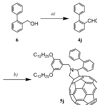
Scheme 3. Reagents and conditions: (a) \text{MnO}_2 , \text{CH}_2\text{Cl}_2 , room temp. (87%); (b) \text{C}_{60} , 3 , ODCB, 180 °C (50%).
